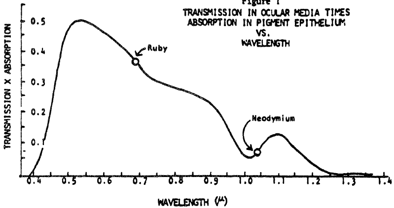
Figure II TRANSMISSION IN OCULAR MEDIA TIMES ABSORPTION IN PIGMENT EPITHELIUM & CHOROID VS. WAVELENGTH
